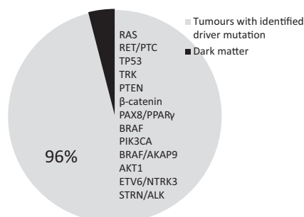
Figure 2 Current status of molecular characterisation of differentiated thyroid cancer.
